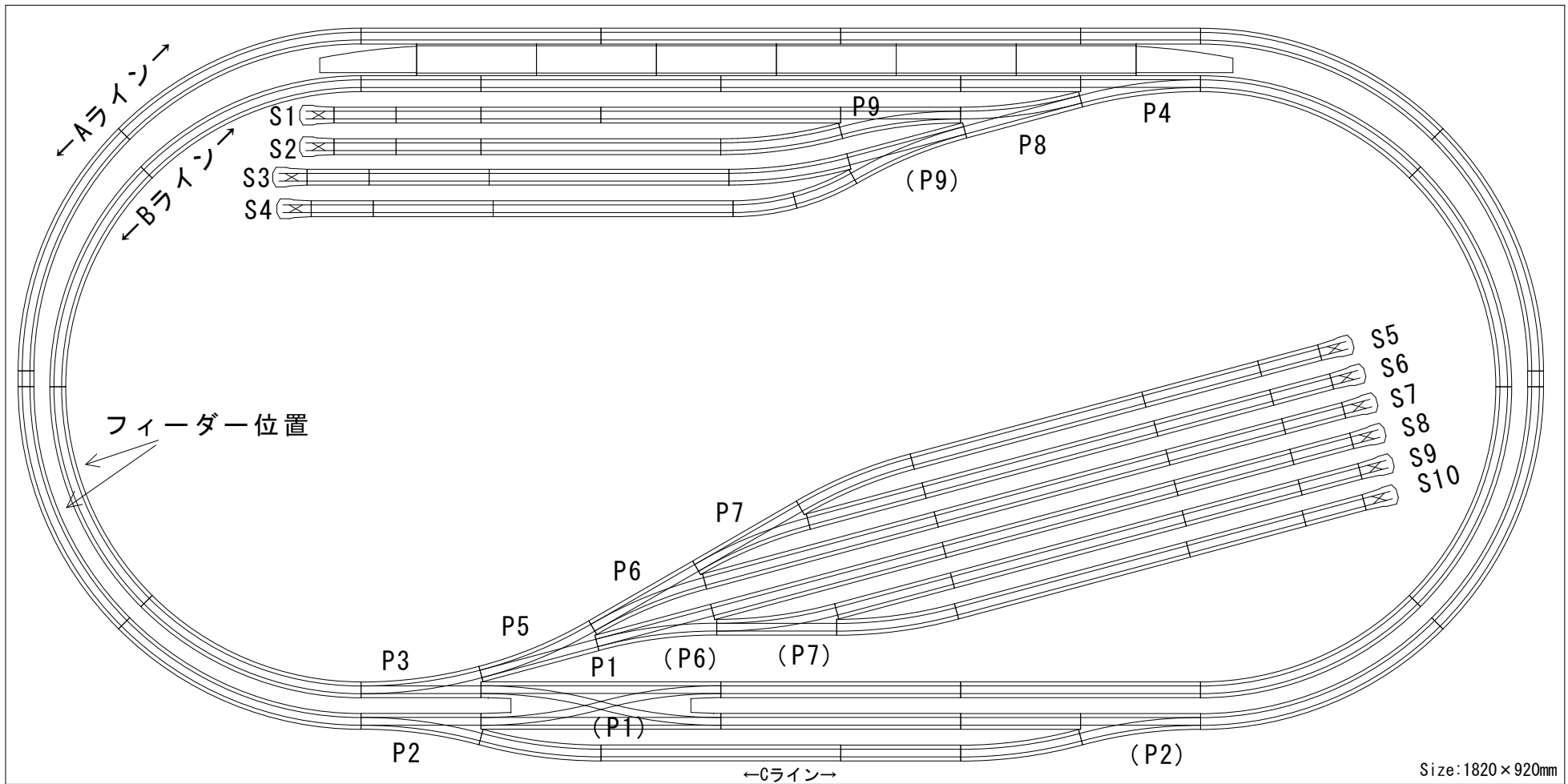
運行計画の各スイッチへの割当 (Assign an operation plan to each switch)
